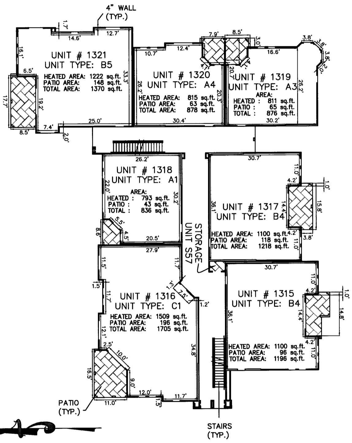
GRAPHIC SCALE
