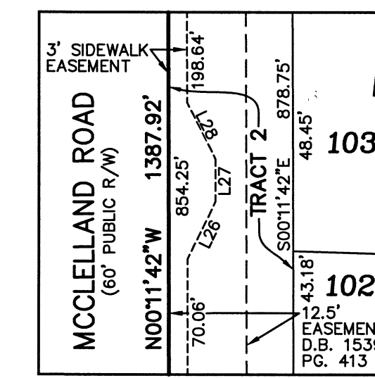
DETAIL "F" (NOT TO SCALE)
