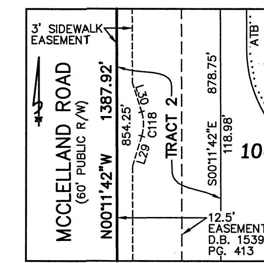
DETAIL "G" (NOT TO SCALE)
