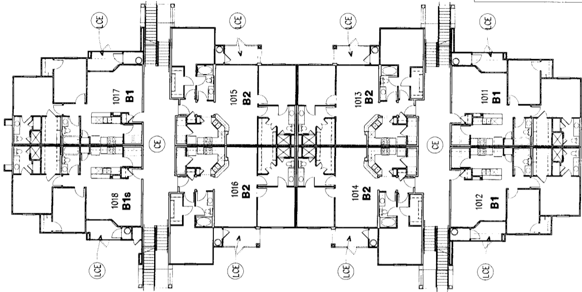
FIRST FLOOR BUILDING TYPE II
