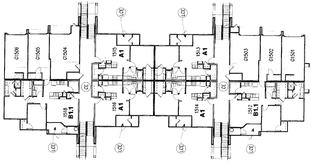
FIRST FLOOR BUILDING TYPE I
