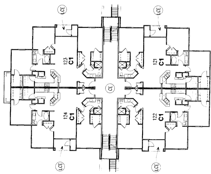
SECOND FLOOR BUILDING TYPE V
