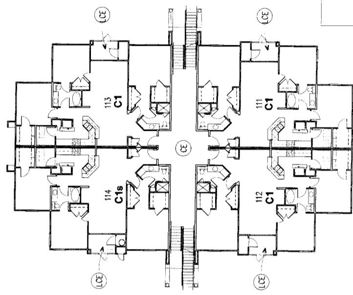
FIRST FLOOR BUILDING TYPE V
