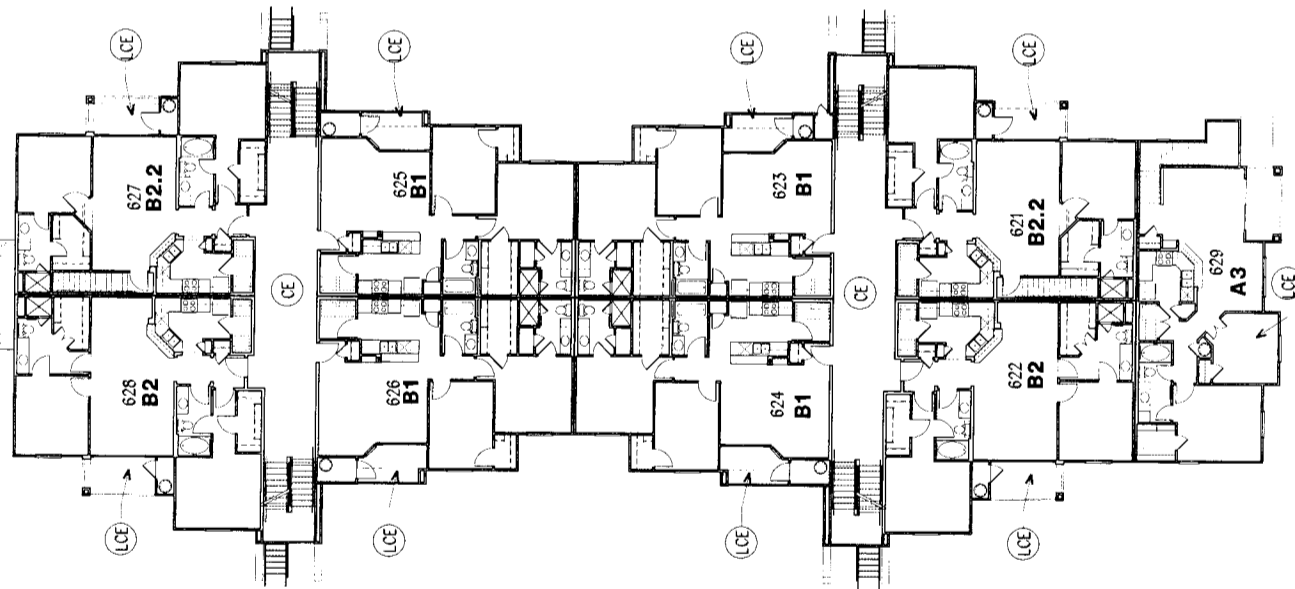
SECOND FLOOR BUILDING TYPE III
