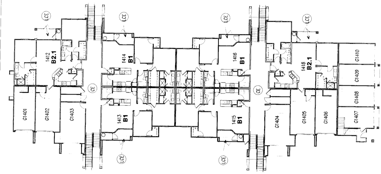
FIRST FLOOR BUILDING TYPE III
