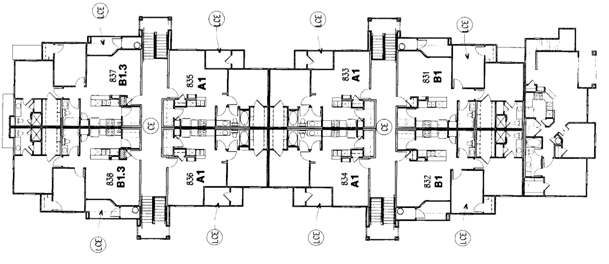
THIRD FLOOR BUILDING TYPE IA
