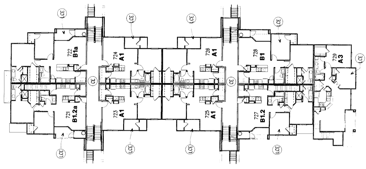
SECOND FLOOR BUILDING TYPE IA
