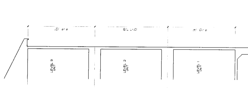
TYPICAL SECTION 3 STORY BUILDING SCALE: 1/8" = 1'-0"
