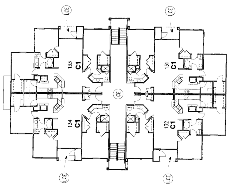
THIRD FLOOR BUILDING TYPE V
