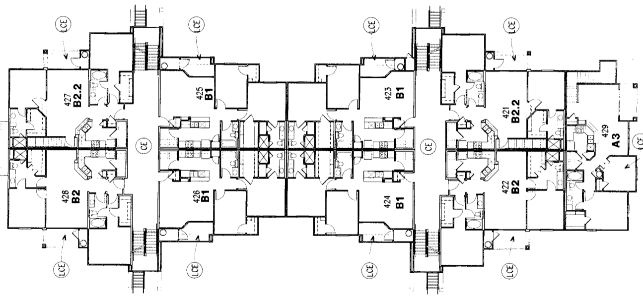
SECOND FLOOR BUILDING TYPE III
