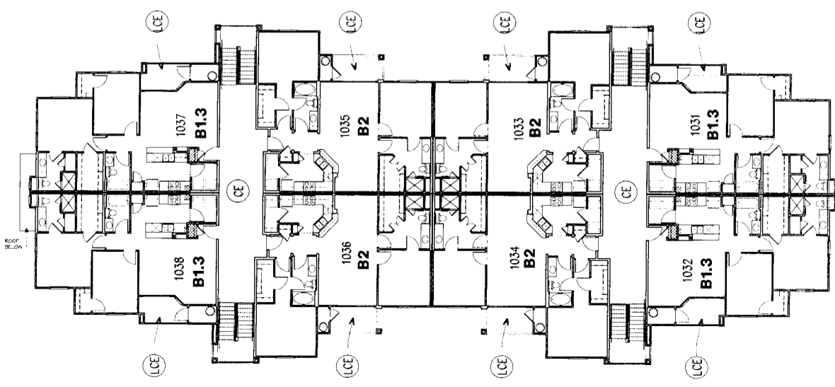
THIRD FLOOR BUILDING TYPE II
