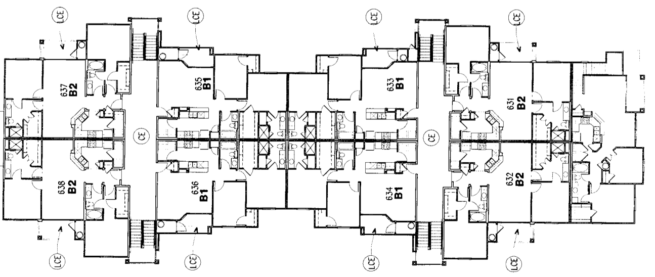
THIRD FLOOR BUILDING TYPE III
