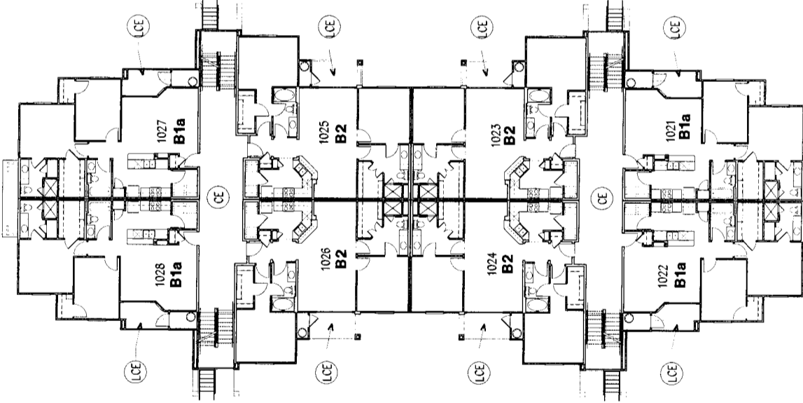
SECOND FLOOR BUILDING TYPE II
