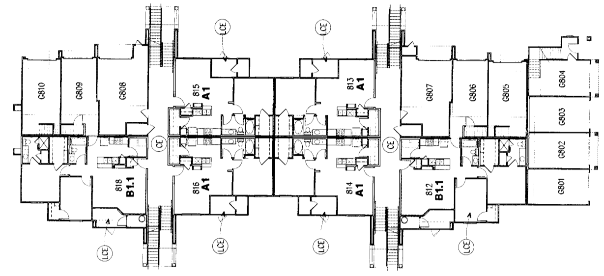
FIRST FLOOR BUILDING TYPE IA
