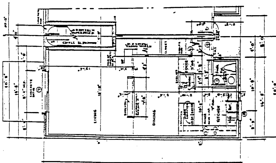
FIRST FLOOR PLAN UNIT TYPE 'F' SCALE: 1/8" = 1'-0" TOWNHOUSE
