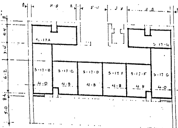
STORAGE AREA, 17th FLOOR
